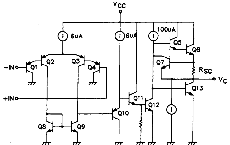
Equivalent Circuit
