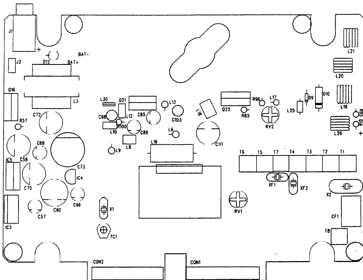
RF Board
